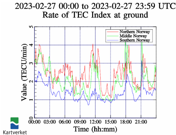
Figure 10: Time series of ground effect of ionospheric disturbances on Feb 27 as characterized by the ROTI products of NMA. These time series are available in the SWESNET service (product I.109).
