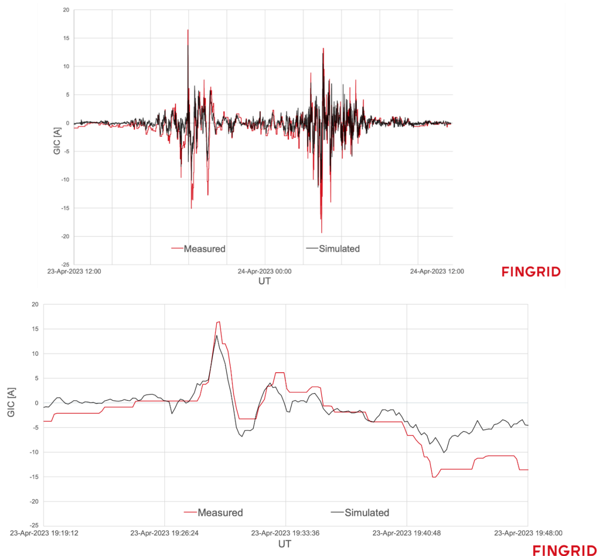
Figure 22: Measured and simulated GIC at one of the GIC recording points in the Finnish power network. Upper panel: the whole modelling interval (23 April 2023, 12:00 - 24 April 2023, 12:00 UT). Lower panel: a closer look on the 23 April 2023, 19:29:30 UT GIC peak (Plots by Fingrid).
