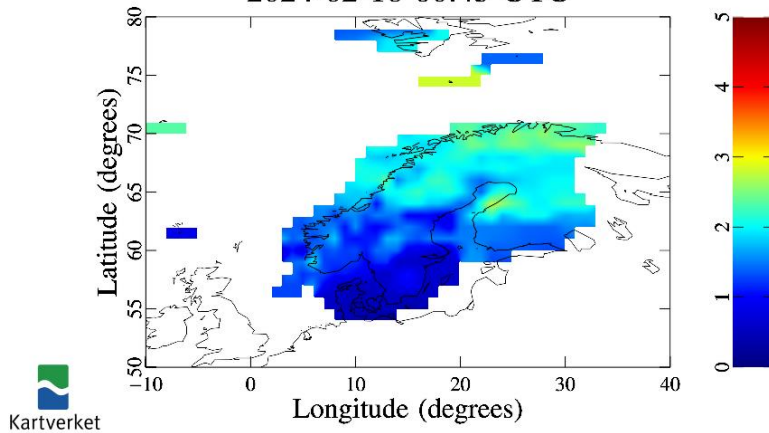
Figure 14: Some machine control system operators are aware of the possibility of space weather impacts and consult space weather monitoring services such as ROTI maps. This map shows an example of moderate-level space weather disturbances (~2 TECU/min) that can result in position errors without triggering built-in warnings in the equipment. This map is available in the SWESNET service (product I.109).
