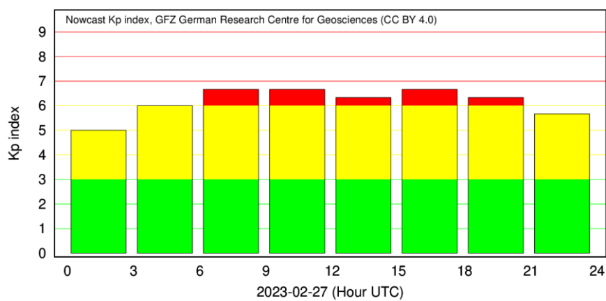
Figure 3: Time evolution of the geomagnetic storm on Feb 27, 2023, as characterized by the global Kp-index. Kp is constructed from the basis of mid-latitude magnetic field measurements. It can have values between 0 and 9. Values in the range of 6-7 are considered as moderate or strong activity. These data are available in the SWESNET service (product G.107).
